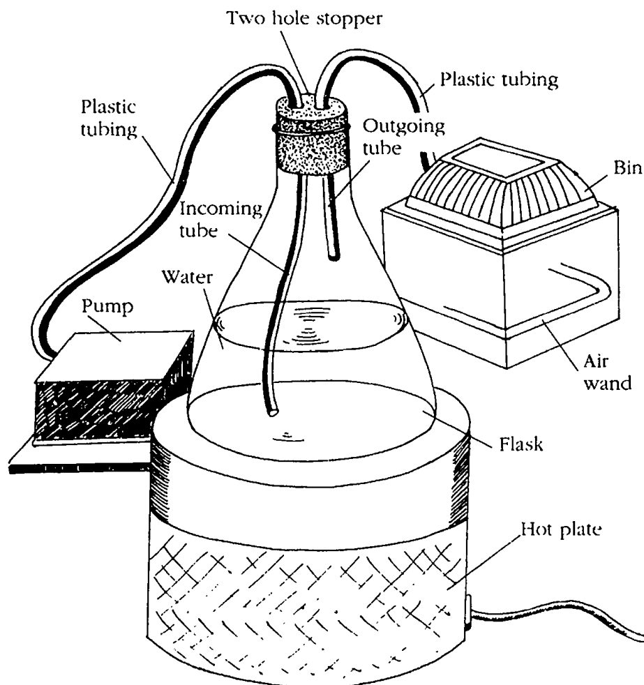
6-1 This apparatus simulates the interior of a compost heap and allows you to control factors such as temperature and moisture.
