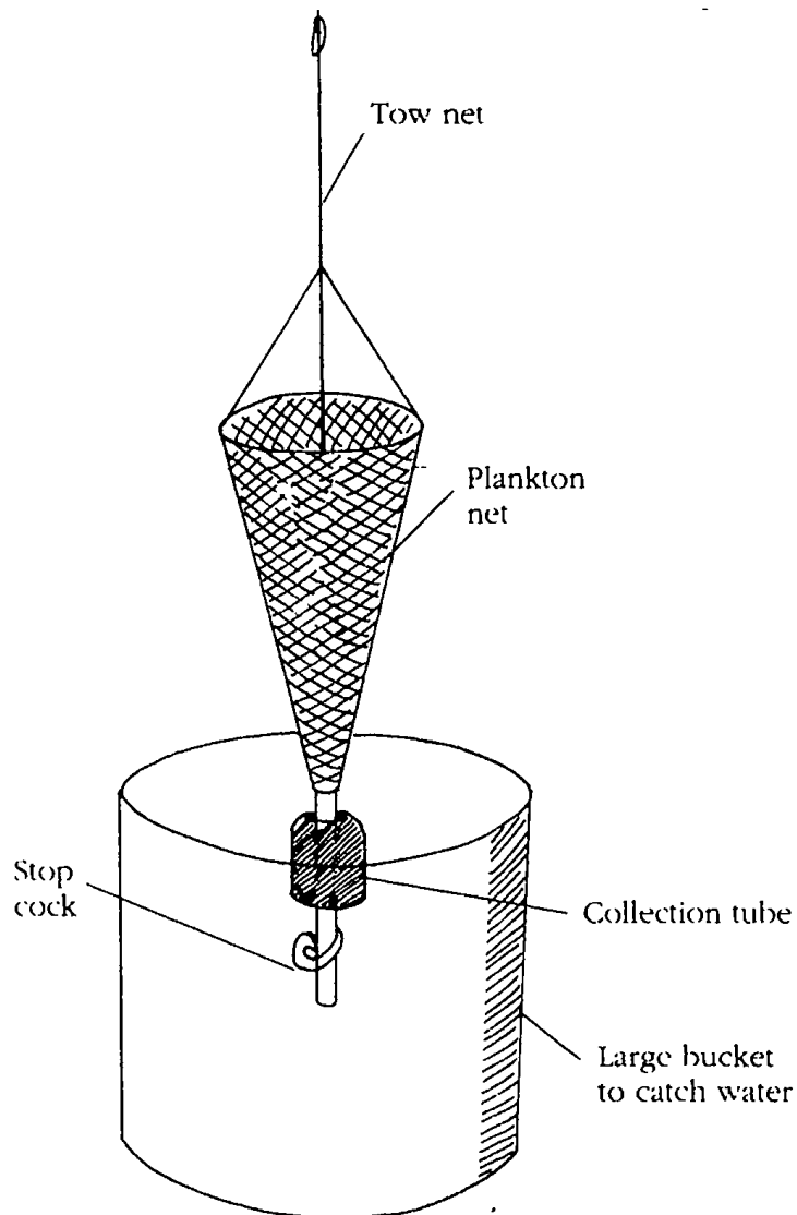
19-2 Use the tow line to hang the plankton collection net upright, so the water samples can be poured through.
