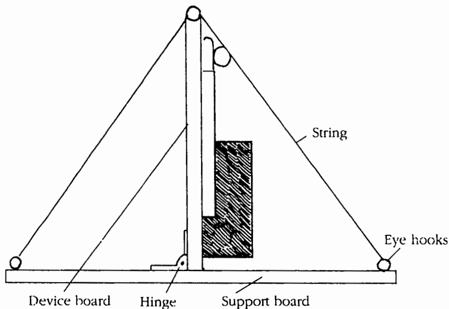
13-2 The device board is mounted with a hinge to the support board. A string running through eye hooks is used to stabilize the apparatus.
